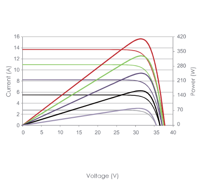
Current-Voltage & Power-Voltage Curves (415W)
